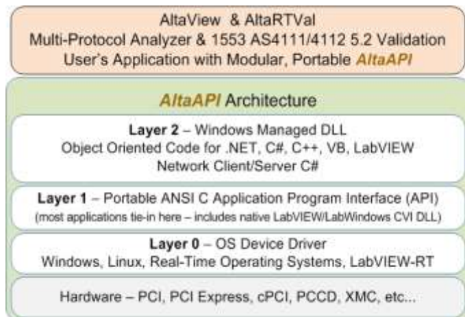
Alta's Advanced Software Architecture
